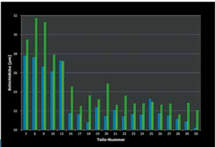
airmatic: Coating thicknesses on various substrates
