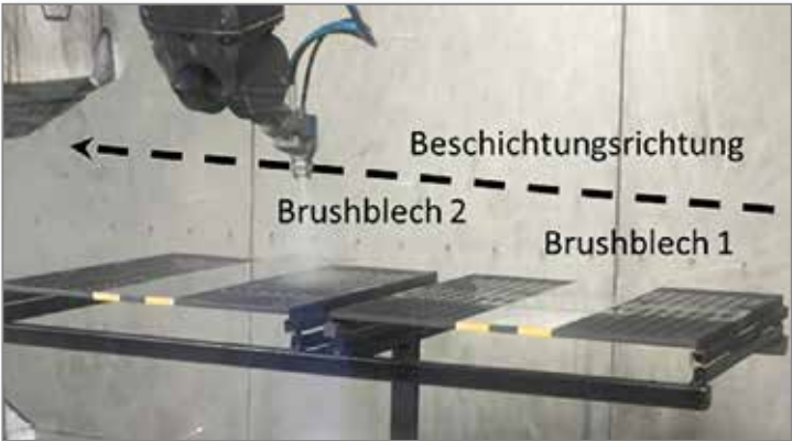
Dynamic spray pattern with robot
